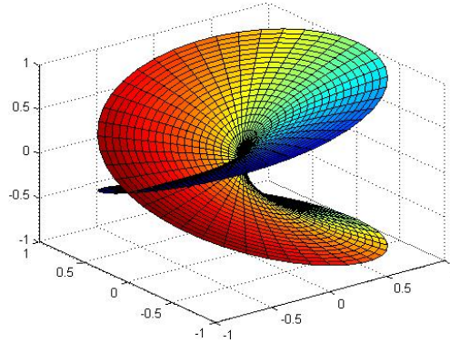
FIGURE 1. Here is the “standard” picture when the ramification number is k = 2 . The graph shown is the neighborhood V of z_0 and f is the projection down onto the xy -plane.
